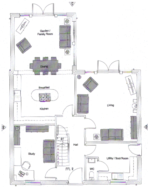
GROUND FLOOR FLOOR AREA 206m 2
